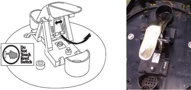
Fuente: Integrated Sensor Suite Installation Manual - DAVIS INSTRUMENTS
